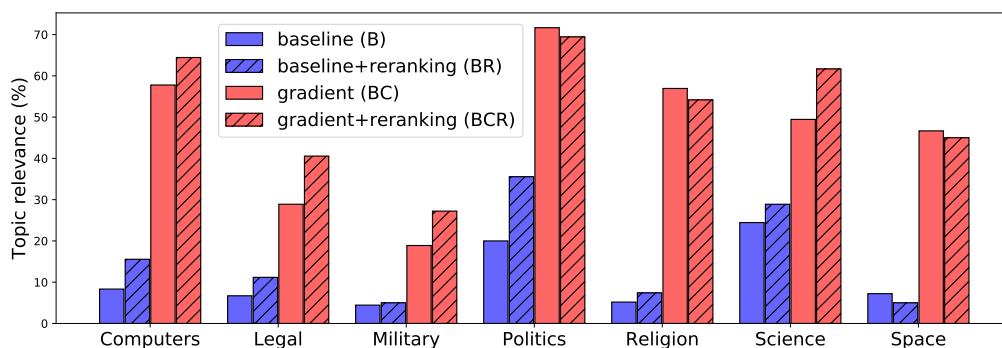
Figure S3: Topic relevance by human evaluation. We can see that taking a PPLM gradient step (B \rightarrow BC) makes a big difference. Reranking is mostly helpful (B \rightarrow BR; BC \rightarrow BCR). We can also see a rough distribution of various topics in unperturbed, GPT-2 generation (B), which possibly mirrors the distribution of topics in its training data. Some topics, like science, naturally appear rather frequently.
