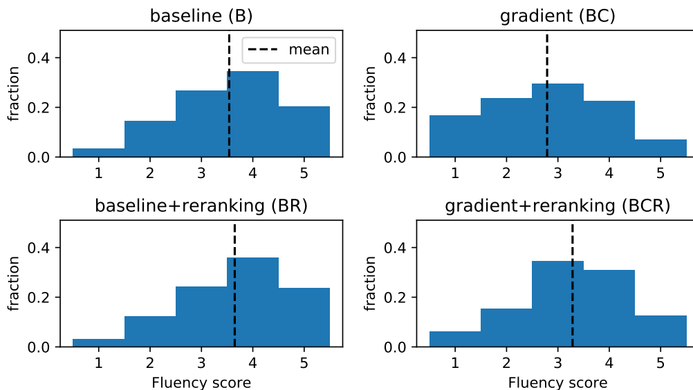
Figure S6: Histogram illustrating the distribution of fluency scores based on controlled generated with PPLM-Discrim from the four methods considered for ablation study. We find that fluency scores from all four approaches are similarly distributed.
