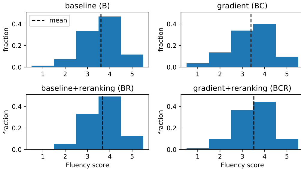
Figure S5: Histogram illustrating the distribution of fluency scores based on controlled generated with PPLM-BoW from the four methods considered for ablation study. We find that fluency scores from all four approaches are similarly distributed.
